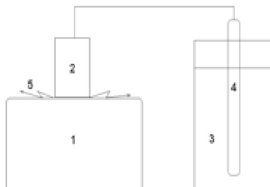
Figure 3: Principle of study of electrophotonic glow of liquids. 1 – EPC instrument; 2 – metal cylinder; 3 – glass with water; 4 – Pt electrode; 5 – sliding gas discharge.
