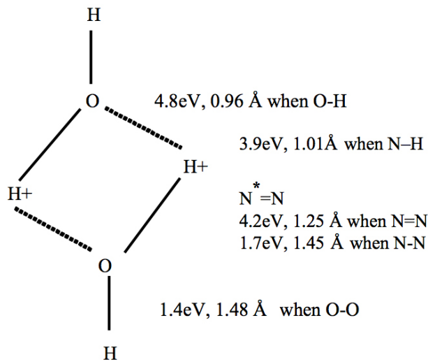
Figure 3: Model for the attack by -N^*=N on an O-H^+ bond (dotted line: hydrogen bond). The values of energy of the covalent bond and the bond lengths are taken from Emsley (1998). The energy of the covalent bond is indicated by converting from kJ/mol into eV .
