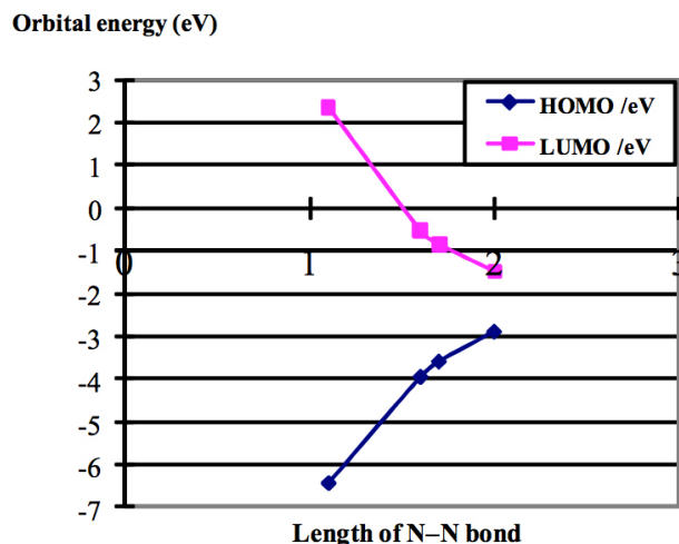
Figure 2: Plots of the orbital energy of the HOMO and LUMO versus the N–N distance (Å).
