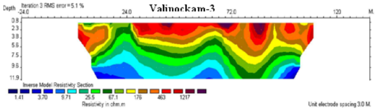
Figure 2.2: 2D Electrical resistivity imaging section show the salt and fresh water interphase at Keelamundal-1 and Keelamundal-2.
